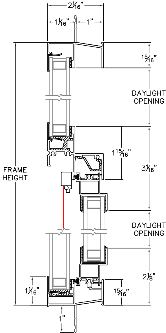
HEAD & SILL
